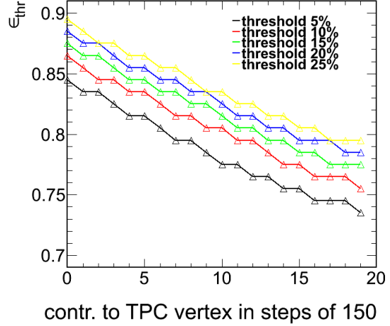
(b) \varepsilon_{thr} vs multiplicity for various thresholds
