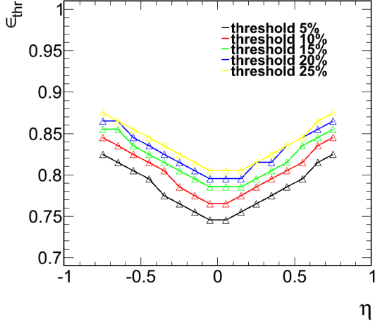
(a) \varepsilon_{thr} vs \eta for various thresholds
