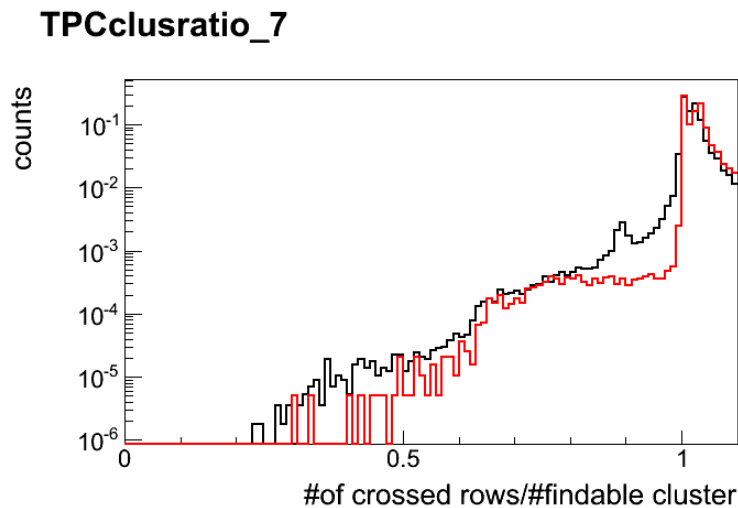
Figure 4: Number of crosses rows divided by number of findable clusters for pp data LHC10d (black) and the corresponding MC sample (red). Shown for tracks with an energy loss of 70-79 and an event multiplicity of 30-45 contributors to the TPC vertex.
