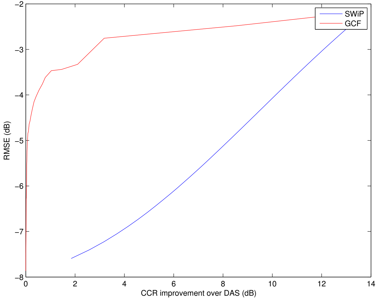
RMSE vs. CCR, SNR=10 dB
