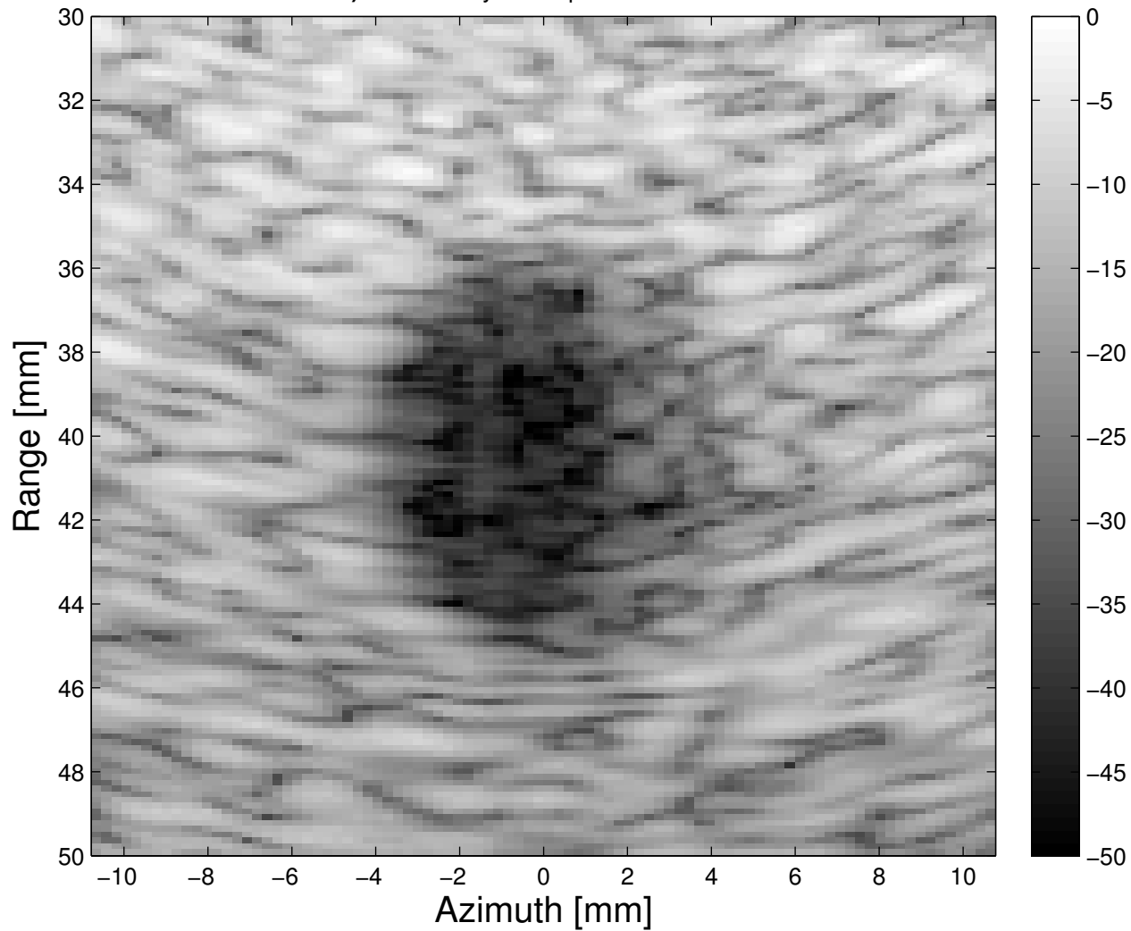
c) Anechoic cyst with phase aberrations
