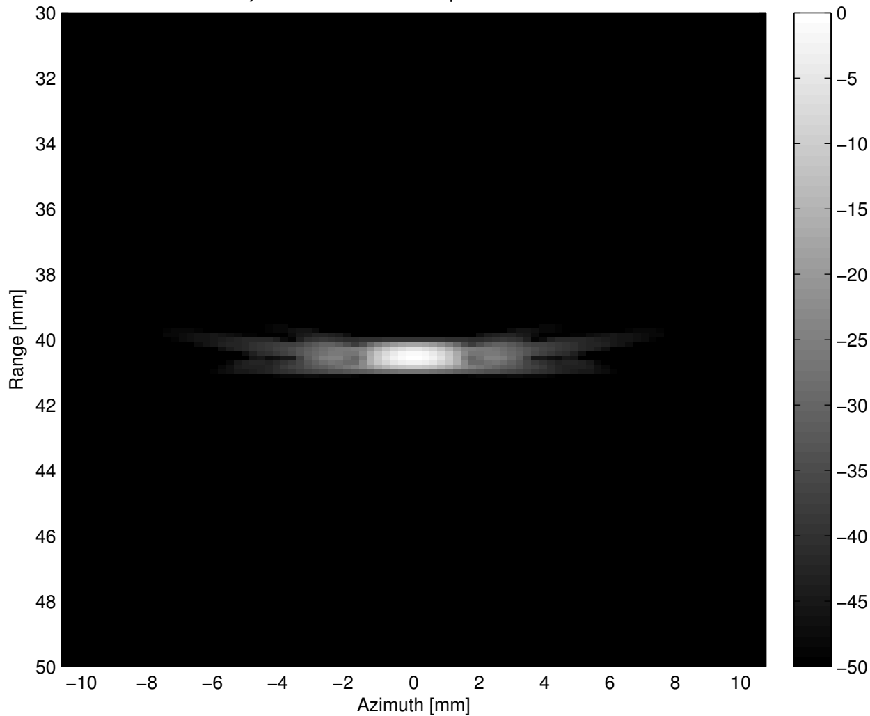
b) Point scatterer without phase aberrations
