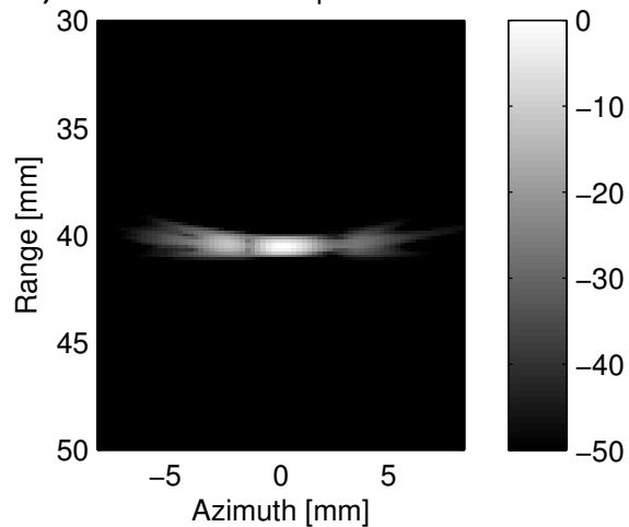
d) Point scatterer with phase aberrations
