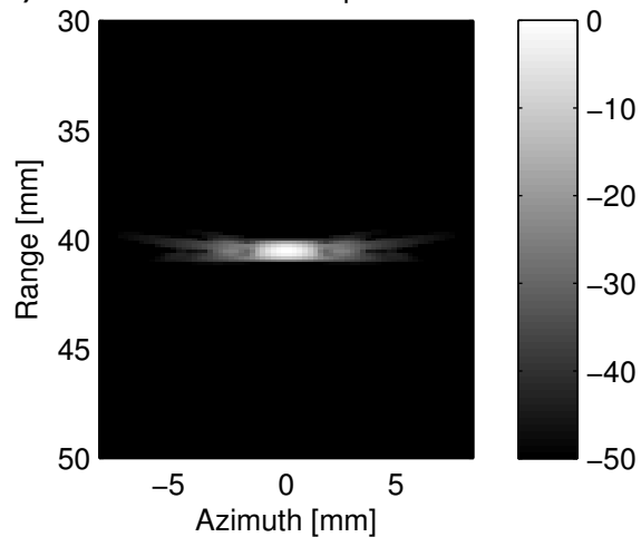
b) Point scatterer without phase aberrations
